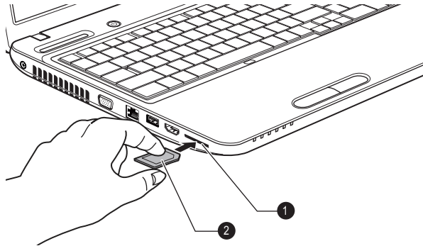
Figure 3-8 Inserting a memory media (Satellite L770/L775/L770D/L775D/satellite Pro L770/L775/L770D/L775D)
